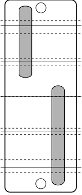
xxM45M - 5 st. split coil - deeper xxM45T - 5 st. split coil - brighter
