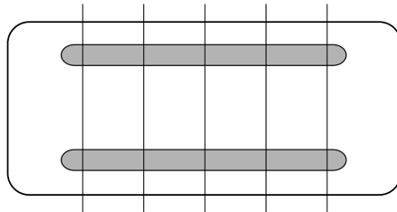
72MV5C - 72mm 5 string dual coil - deep tone 72MV5K - 72mm 5 string dual coil - bright tone
