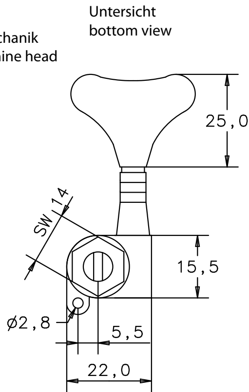
rechte Mechanik right machine head
