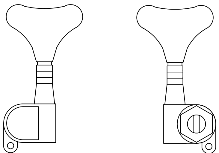
rechte Mechanik right machine head
